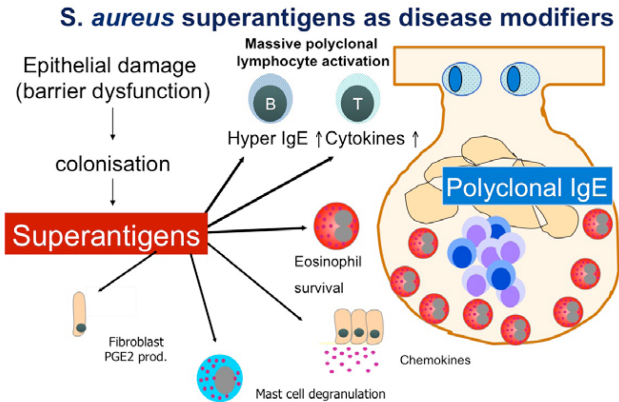
Figure 4.2.1.: Overview of the 'superantigen hypothesis' of CRS.
